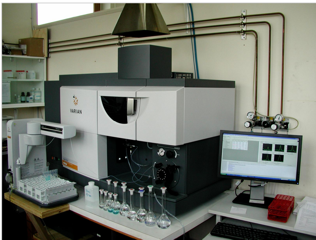
ICP-OES Analysis equipment
